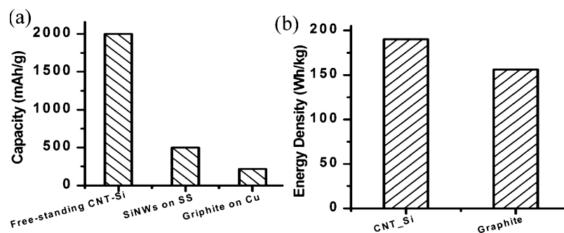
Figure 6. (a) Specific capacity for different anode systems, including the mass of the electrode material and the current collector. (b) Specific energy density comparison at whole battery level, including all the device components.
