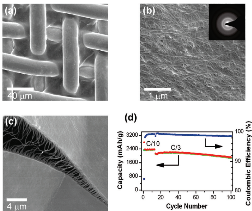
Figure 2. (a) SEM image of a CNT-Si film supported by a SS 500 mesh. (b) Zoom-in SEM of Figure 1a. Inset is a SAED image of the film. (c) SEM image of a broken film supported by SS mesh. (d) Charge (red) and discharge (green) capacity and Coulombic efficiency (blue) versus cycle number for a half cell using a SS mesh supported CNT-Si film as the working electrode cycled between 1–0.01 V.
